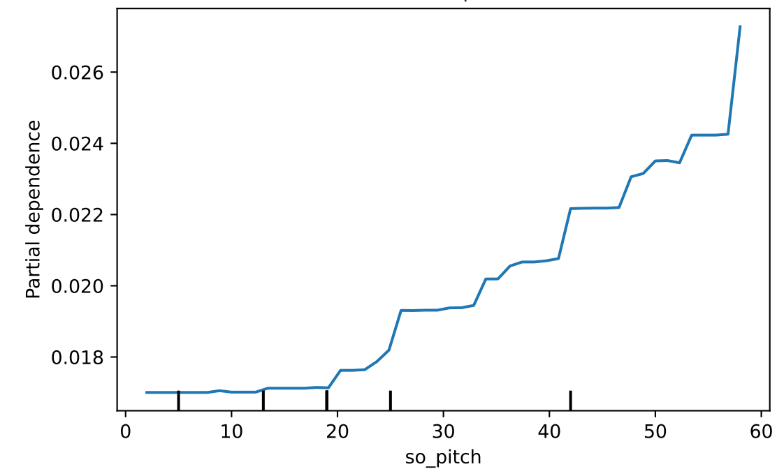
PDP: SO (pitch)
